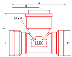
RT 908 Raccordo a T FxMxM.
