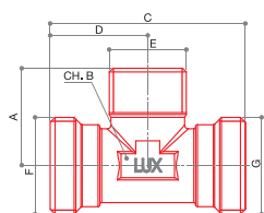
RT 907 T fitting MxMxM.
